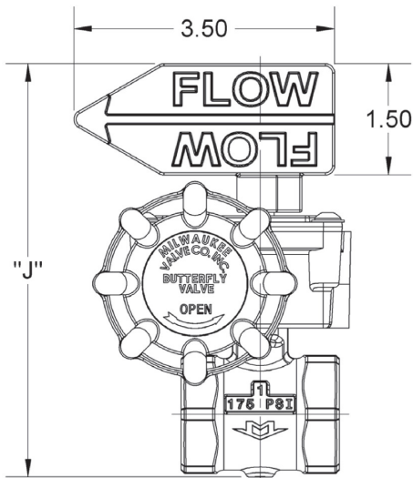
BB-SC100 and BBSCS-02 (Threaded Ends) Sizes 1", 1-1/4", 1-1/2", 2", 2-1/2"
